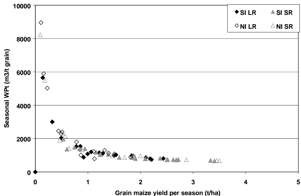
Figure 4. Relation between yield and water use in m^3 per ton of grain for maize.
